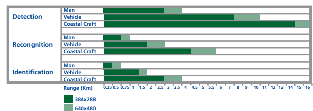
DAGIR range performance chart (clear air 20km)
